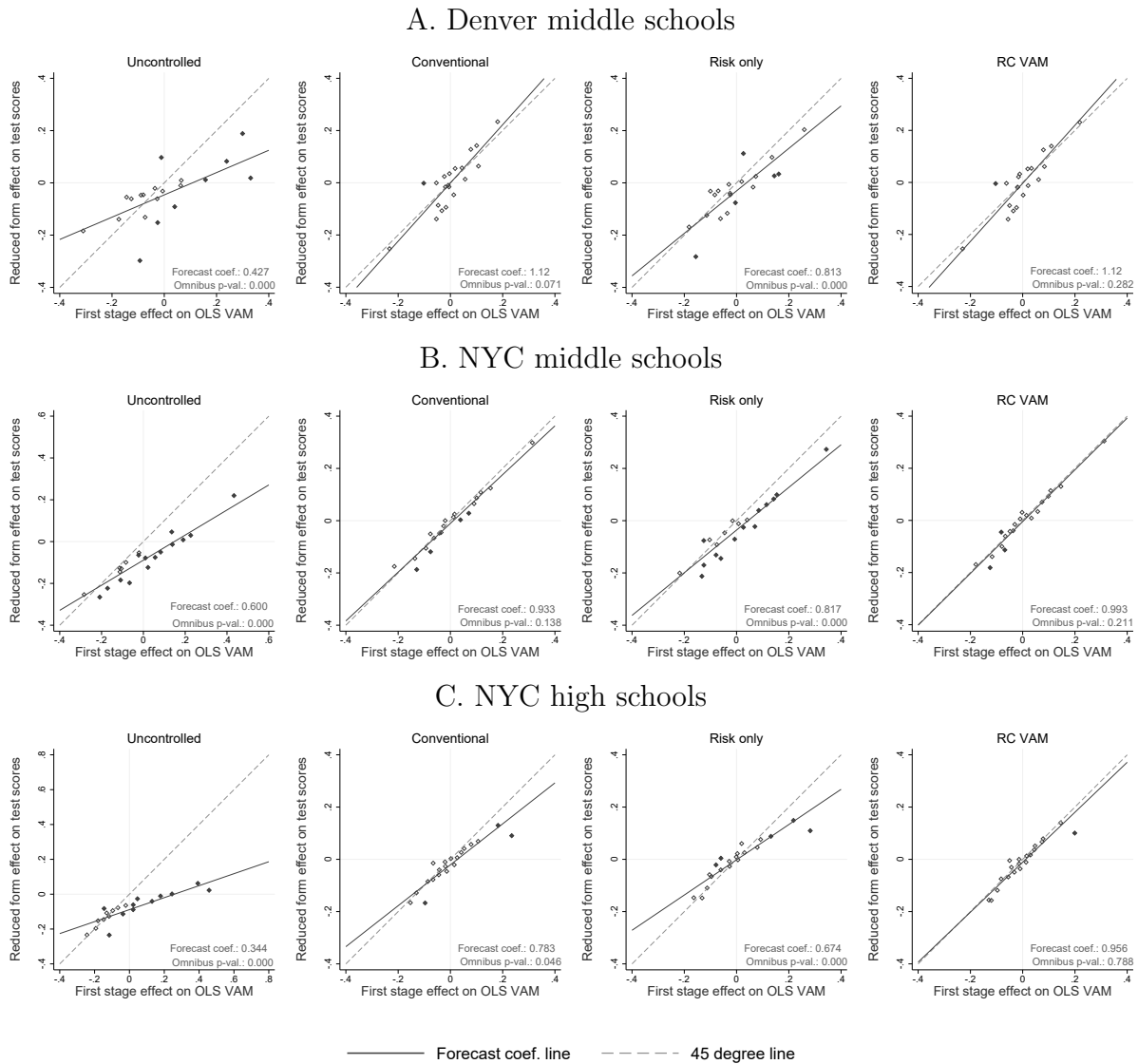
Figure 1. Visual Instrumental Variables Tests for Bias (Math)
